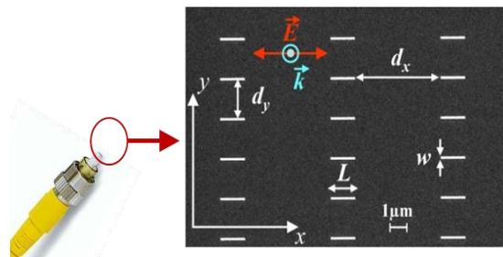
Fig.1 : Schematic view of the envisioned integration of a plasmonic array in a fiber architecture
